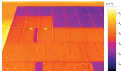
Corroded cell connections on two Modules lead to partial failures
