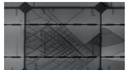
Electroluminescence image of a cell with many microcracks
